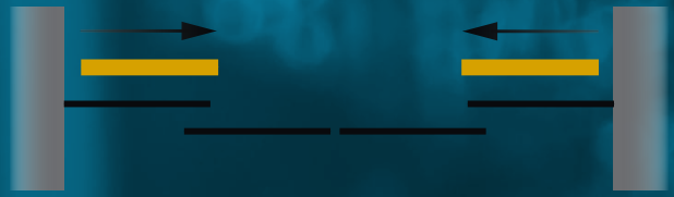
GSW 17 (centre opening) + 2 sliding panels, 2-track
